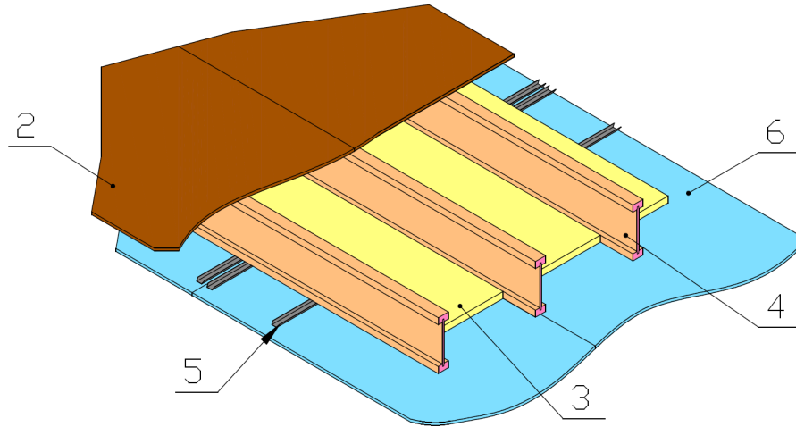
FIGURE 4 – 1-Hour Fire-Rated Floor-Ceiling or Roof-Ceiling Assembly
