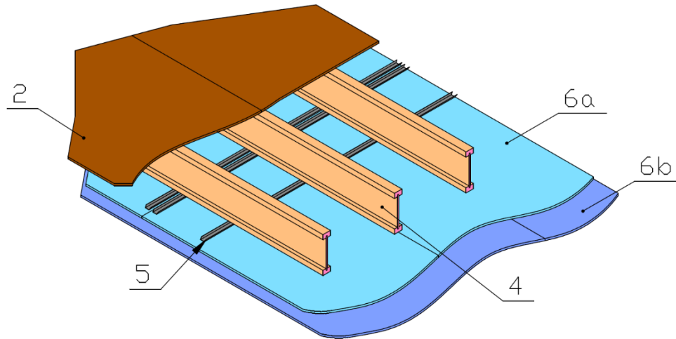
FIGURE 3a – 1-Hour Fire-Rated Floor-Ceiling or Roof-Ceiling Assembly
