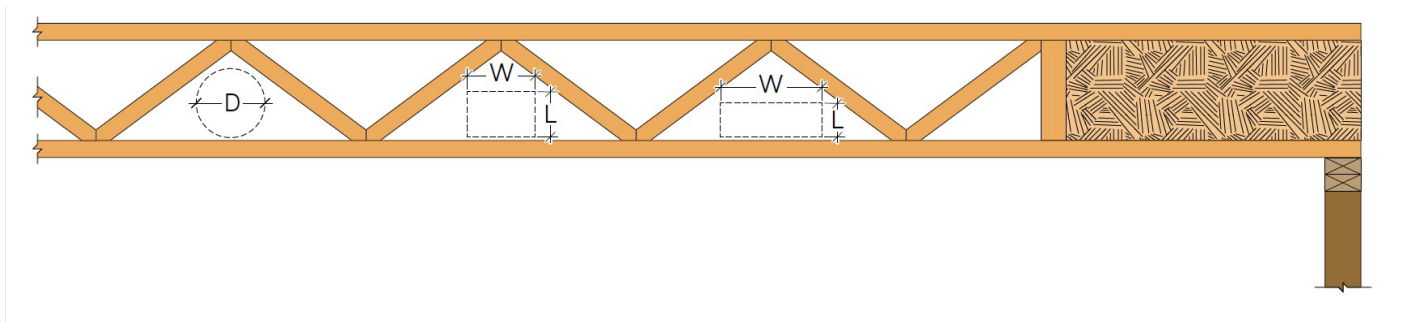
FIGURE 3- Mechanical Clearances
